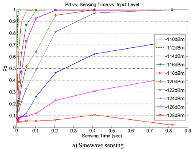
a) Sinewave sensing
